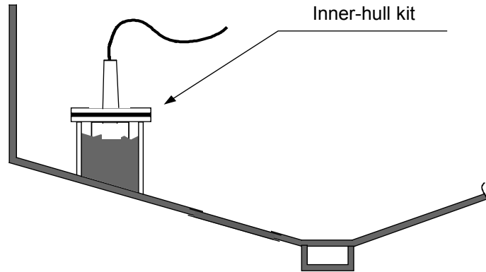
Figure 5.6 Installation of Transducer
