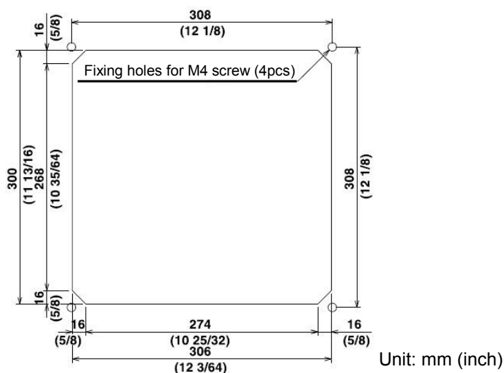
Fig. 5.5 Work of flush-mount installation hole
