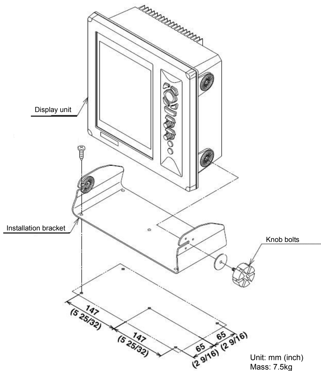
Fig. 5.2 Desk-top installation
