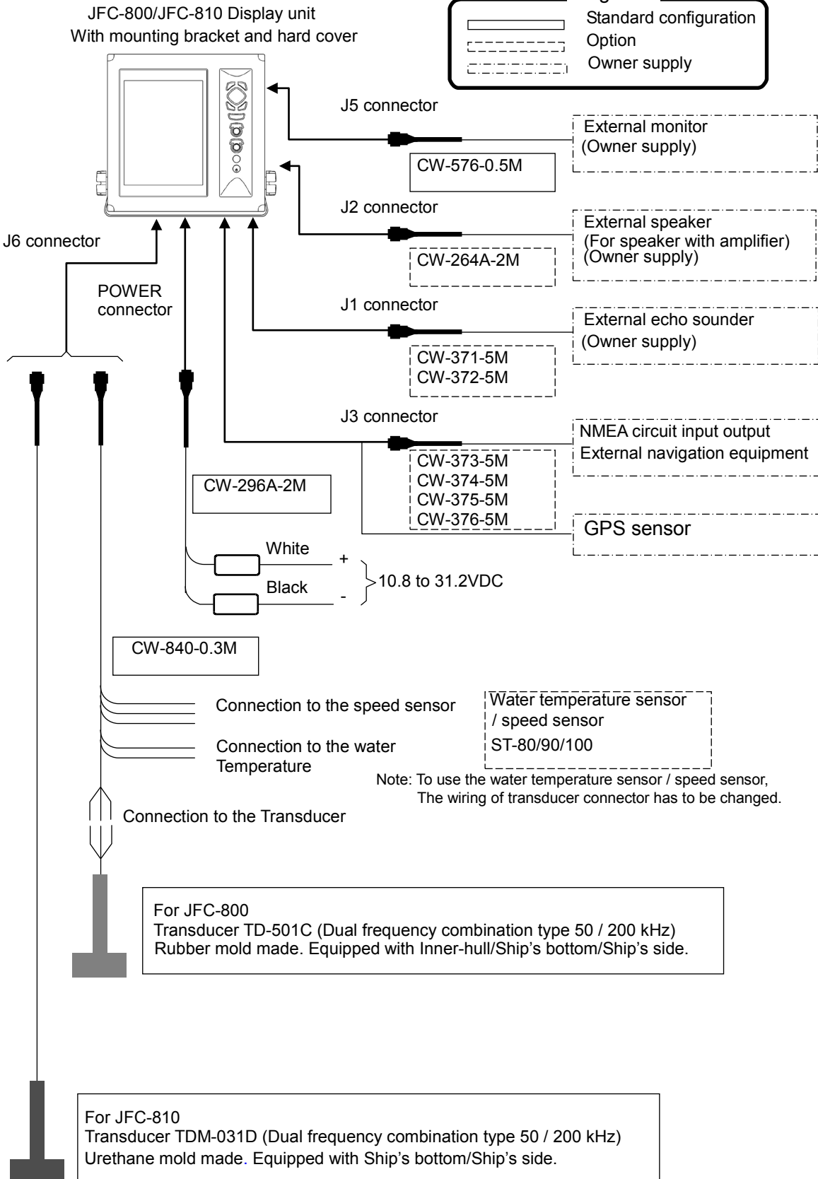
Connection Diagram
